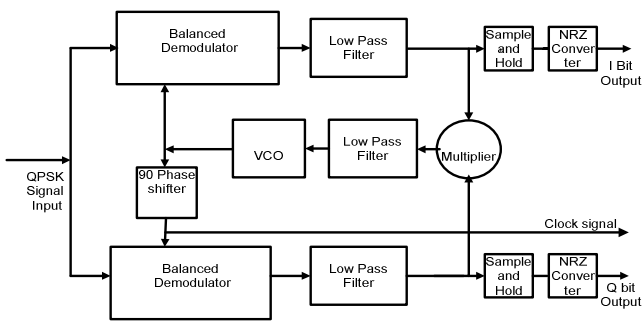
Fig. 3. QPSK Demodulator. The input is QPSK signal & output is I-Bit & Q-Bit.
