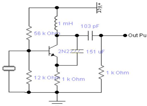
Fig. 14. Carrier Signal Generator
