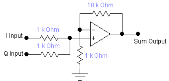
Fig. 12. Summing Amplifier
