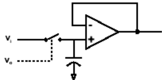
Fig.17. Sample &amp; Hold Circuit
