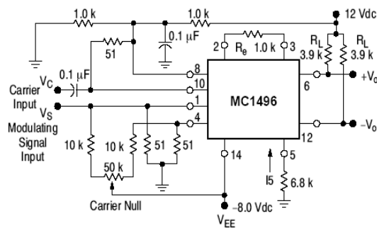
Fig.9. Balanced Modulator typical Circuit.
