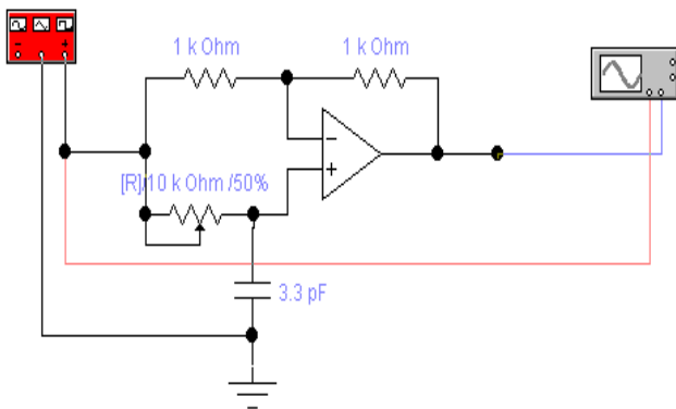
Fig.10. Phase Shifter Diagram
