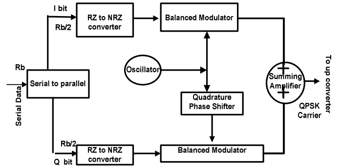
Fig.2. Block Diagram of Quadrature Phase Shift Keying (QPSK) Modulator.
