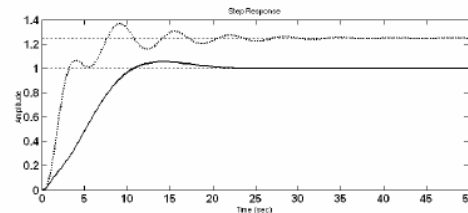
Fig. 6. a, Table II, K_p = 0.04
