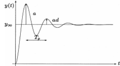
Fig. 4 System with underdamped step response used for identification of the process.
