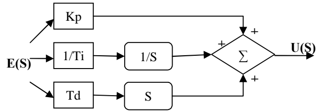
Fig.1. Standard PID Controller
